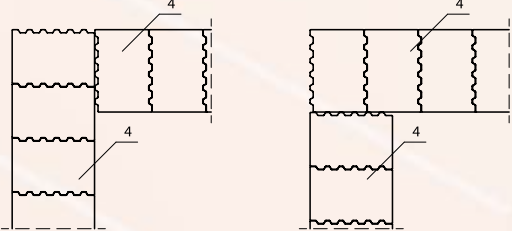
POROTHERM 38 P+W
