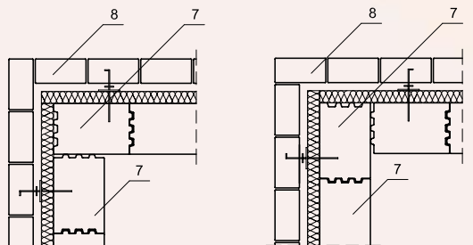
POROTHERM 25 P+W
