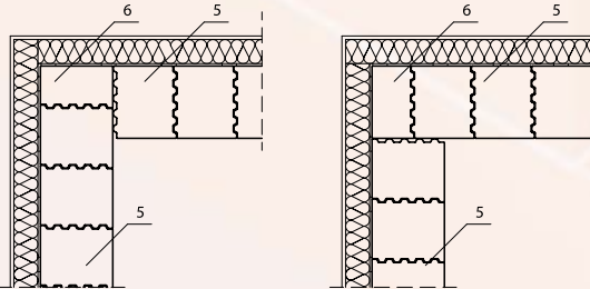
POROTHERM 30 P+W
