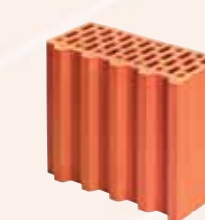
POROTHERM 30 1/2 P+W
