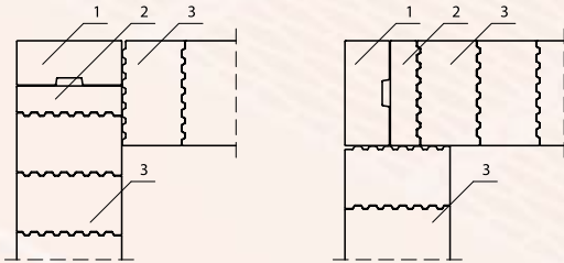
POROTHERM 38 P+W
